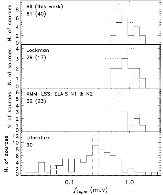
Fig. 6.— 24\mu\text{m} flux distribution of sources with f_{1.2\text{mm}} > 2\sigma (solid line) and with f_{1.2\text{mm}} < 2\sigma (dotted line). From top to bottom, all MAMBO/SWIRE sources, those in the Lockman Hole, those in the other fields, and those in the literature (Frayer et al. 2004b; Egami et al. 2004; Borys et al. 2005; Chapman et al. 2004; Greve et al. 2004; Pope et al. 2006). The dashed histogram represents the literature sources that are not detected at 24\mu\text{m} for which we assumed a 5\sigma upper limit ( 250\mu\text{Jy} for 12 sources in the SWIRE fields, and 26\mu\text{Jy} for 1 GOODS SMG, and 506\mu\text{Jy} for 3 more GOODS SMGs). The total number of sources is annotated on the upper left corner in each panel. The value in parenthesis represents the number of sources with f_{1.2\text{mm}} < 2\sigma .
