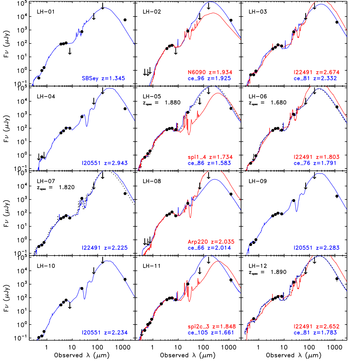
Fig. 13.— Optical-IR SEDs of MAMBO sources in the Lockman Hole field. The solid curves represent different fits to the optical-MIR data (up to 24\mu\text{m} ). Blue, red and green curves correspond to fits with increasing \chi^2 . The template name and photometric redshifts of each fit are annotated. The dotted curve corresponds to the best-fit template plotted at the spectroscopic redshifts. The source ID number, and the spectroscopic redshift when available, are reported on the upper left corner in each panel. Downward arrows represent 5\sigma upper limits at optical and infrared wavelengths, and 3\sigma upper limits at 1.2\text{mm} .
