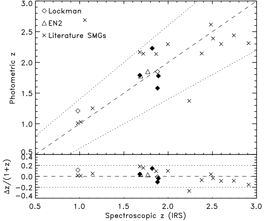
Fig. 3.— Comparison between photometric and spectroscopic redshifts from IRS (Lonsdale et al., in prep. Weedman et al. 2006) of the 8 SWIRE/MAMBO sources with available spectroscopic redshifts (diamond and triangles). Dotted lines represent 20% agreement in (1+z) . Full symbols represent sources with f_{1.2\text{ mm}} > 2\sigma , and empty symbols sources with f_{1.2\text{ mm}} < 2\sigma . Diamonds represent LH sources, and triangles sources in the other three SWIRE fields. Crosses represent 15 sources from the literature sample of SMGs with available spectroscopic redshifts, a 24\mu\text{m} detection, and exhibiting a peak in the IRAC bands.
