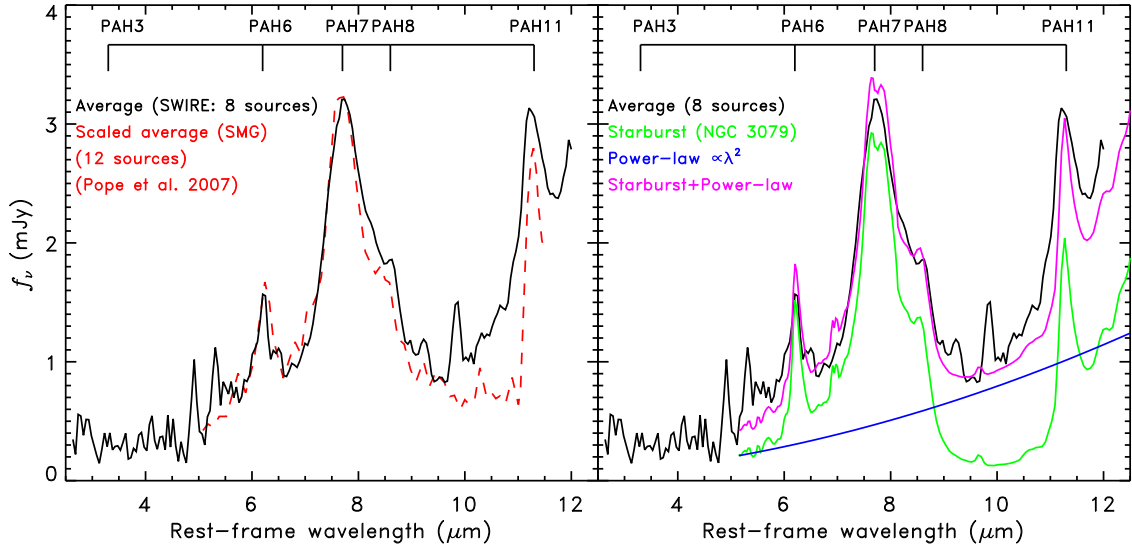
Fig. 9.— Average IRS spectrum of the 8 SWIRE sources with available IRS spectra (black solid curve). Left panel: Also shown the composite spectrum of 12 SMGs from the HDFN (Pope et al. 2007) after scaling it to match the SWIRE average spectrum (red dashed curve). Right panel: IRS spectrum of a starburst (NGC 3079; green curve), a power law model with spectral index 2 representing warm dust continuum emission (blue curve), and the sum of the two (magenta curve). The expected locations of PAH emission features are labeled in both panels.
