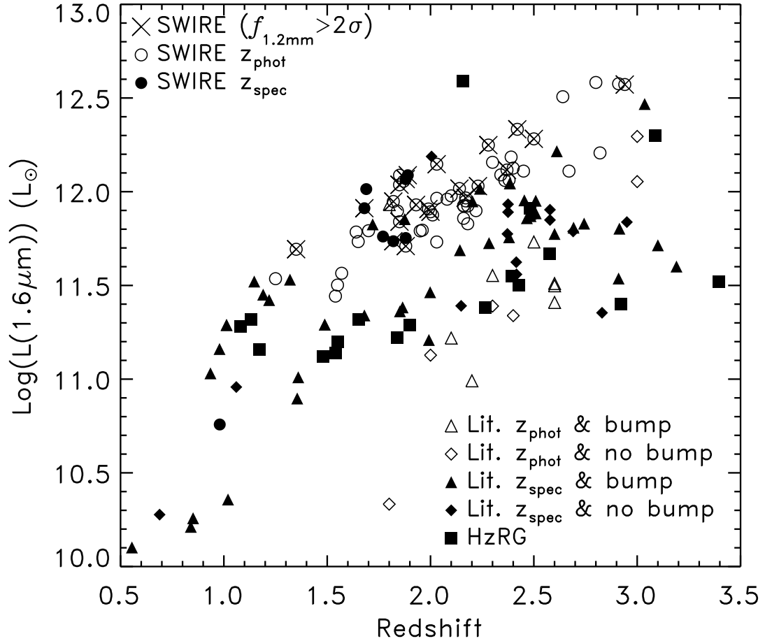
Fig. 12.— Monochromatic luminosity at 1.6 \mu\text{m} in the rest-frame for SWIRE/MAMBO sources (circles), for literature SMGs (triangles and diamonds), and for high- z radio galaxies (squares). Full symbols represent sources with spectroscopic redshifts and open symbols with photometric redshifts. Triangles represent sources with a typical stellar bump in the IRAC bands and diamonds sources where the bump is not present or not detected. Large crosses are overplotted on SWIRE/MAMBO sources with f_{1.2 \text{ mm}} > 2\sigma .
