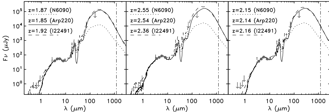
Fig. 2.— Fits of 3 SWIRE/MAMBO sources with the 3 starburst templates used to predict 1.2mm flux densities, Arp 220 (solid curve), NGC 6090 (dotted curve), and I22491 (dashed curve). Downward arrows represent 5\sigma upper limits. The vertical dot-dashed line represents the 1.2 mm wavelength.
