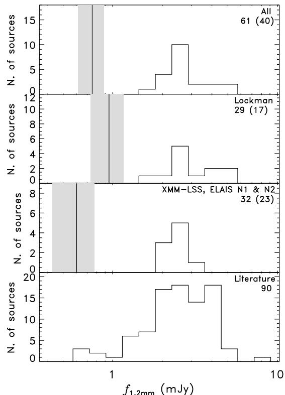
Fig. 5.— 1.2\text{ mm} flux distribution of sources with f_{1.2\text{mm}} > 2\sigma (histogram). The mean and mean standard deviation of the sources with f_{1.2\text{mm}} < 2\sigma are shown as a vertical solid line and a gray shaded area. From top to bottom, all MAMBO/SWIRE sources, those in the Lockman Hole, those in the other fields, and those in the literature (Frayser et al. 2004b; Egami et al. 2004; Borys et al. 2005; Chapman et al. 2004; Greve et al. 2004; Pope et al. 2006). The total number of plotted sources is annotated and in parenthesis the number of sources with f_{1.2\text{mm}} < 2\sigma is given.
