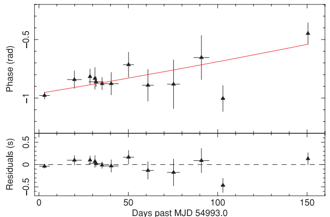
Figure 2. Top panel: 2–10 keV RXTE/PCA (binned at 10 d) and Swift /XRT pulse phase evolution with respect to the period measured by Göğüş et al. (2009a) as a function of time. The red solid line represents the phase-coherent timing solution (discussed in Section 4). Bottom panel: time residuals with respect to the timing solution.
