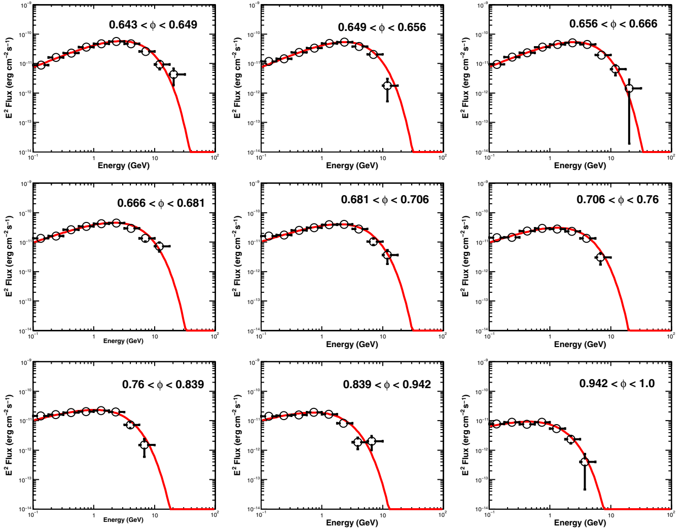
Figure 12. Phase-resolved SEDs of the Geminga pulsar in the phase range \phi = 0.643 – 1.0 . (A color version of this figure is available in the online journal.)
