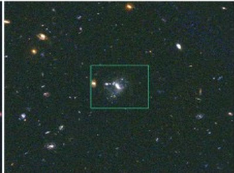
Space: HST (2.4m)
