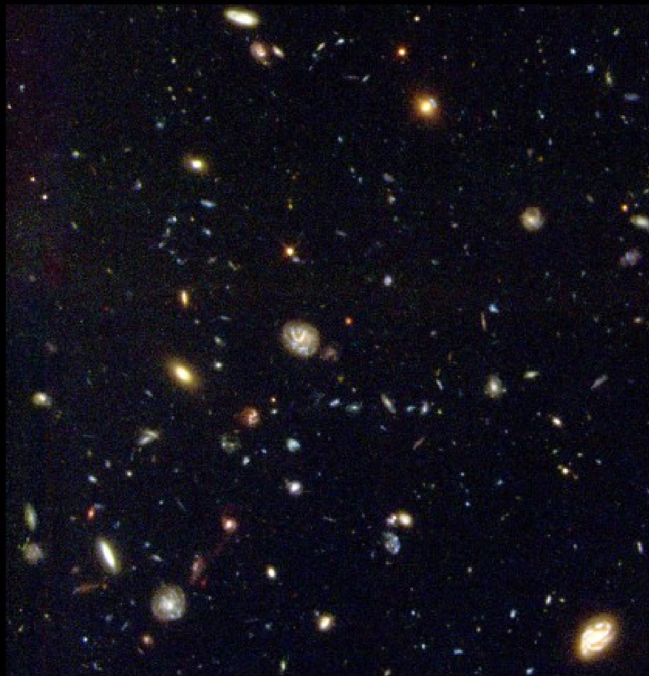
1998: Hubble Deep Field South, 10 d of total observ- ing time!
