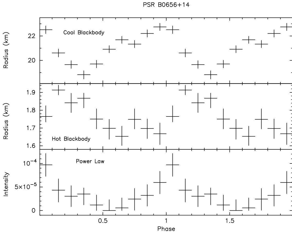
Fig. 12.— The parameters best fitting the phase-resolved spectra of PSR B0656+14 are plotted as a function of the pulsar phase defined as in Fig. 5. Both cool and hot blackbody emitting surfaces evolve throughout the pulsar phase following a sinusoidal pattern showing an overall \sim 10\% modulation (wrt. the average values) on the emitting radii value. Note the marked anti-correlation between panel 1 and panel 2 with the hot blackbody peaking in correspondence of the cool blackbody minimum. The power law component has a different phase trend wrt. the thermal components, with a single, sharper peak.
