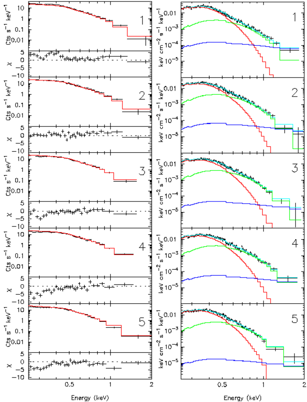
Fig. 9a.— Phase-resolved spectra of PSR B0656+14. Photons have been selected in correspondence of the phase intervals marked in Fig. 6. Phase intervals from 1 to 5 are shown here; phase intervals 6-10 are shown in Fig. 9b. Upper panels on the left column present, for each phase interval, the observed spectrum (data points) compared to the best fit model (solid line) of the phase-integrated spectrum (upper plots); lower panels show the difference between data and such model in units of statistical errors. To ease the visibility of the deviations of phase-resolved spectra from the averaged spectrum template, spectral channels have been rebinned. Panels on the right column show, for each phase interval, the unfolded spectrum together with its best fit model. The model components are also plotted (color code as in Fig. 2). An animated version of Figures 9a/b, 10a/b and 11a/b is available at http://www.mi.iasf.cnr.it/~deluca/3musk/
