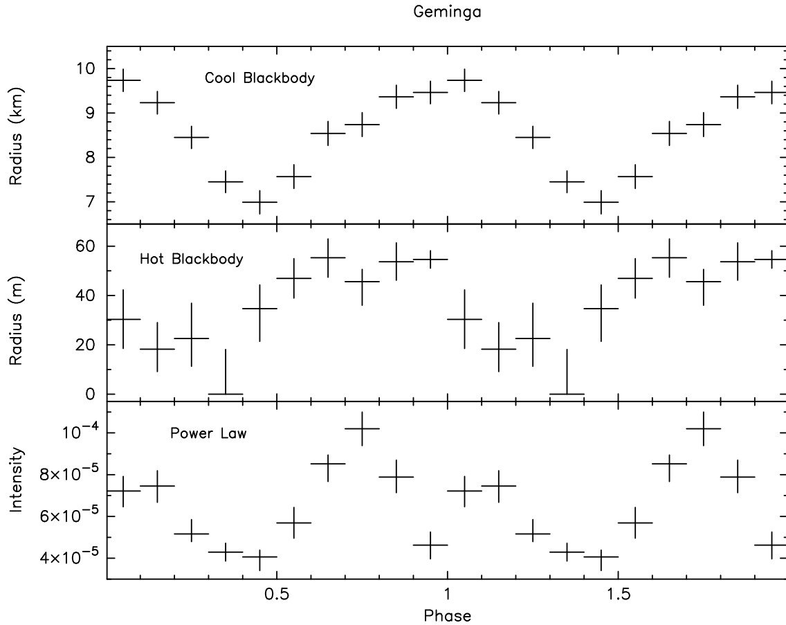
Fig. 14.— Same as Fig.12 and Fig.13 for the case of Geminga. The figure is adapted from Caraveo et al.(2004) (see their Figure 4), according to the choice of phase adopted in this work. The cool blackbody component shows a \sim 15\% modulation (wrt. the average value) of its emitting radius, with a sinusoidal profile. Conversely, the hot blackbody is 100% modulated, and disappears for 1/10 of the pulsar period. The power law component has a remarkably different, double-peaked phase profile and shows a significant unpulsed fraction.
