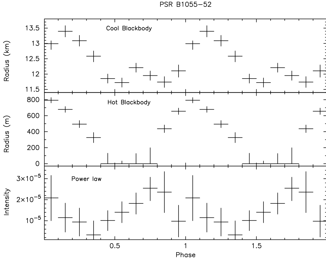
Fig. 13.— Same as Fig.12, for PSR B1055-52. While the cool blackbody emitting radius shows a <10\% modulation (wrt. the average value), the hot blackbody component show a dramatic, 100\% modulation since its contribution is null in 4 of the 10 phase intervals. Note that for PSR B1055-52 the two thermal components have a similar time evolution, with a phase shift as low as \sim 0.1 . The power law component has a different modulation; it is difficult to assess whether its profile is single-peaked or double-peaked, owing to the lower signal to noise in the high energy portion of the spectra.
