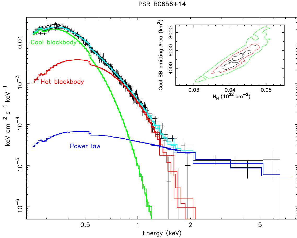
Fig. 2.— Same as Fig. 1 for the case of PSR B0656+14. Data from pn (both Small Window and Fast Timing mode) and MOS1 are plotted (black points). Detailed values of the best fitting parameters are reported in Table 3.
