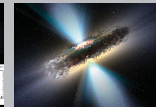
Extragalactic Giant Black Holes
