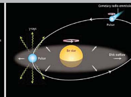
Pulsars in Binary Systems
