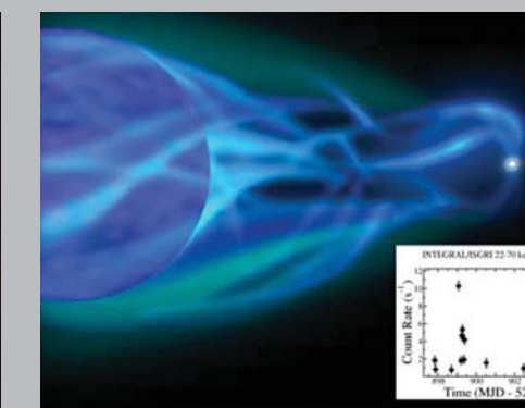
Gamma Ray Transients with Supergiant Companions
