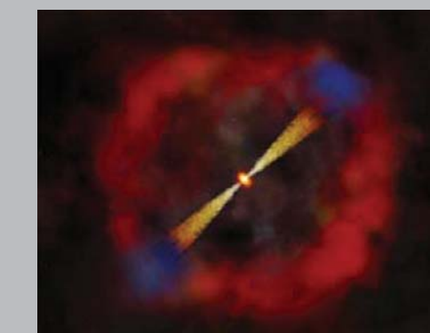
Mysterious Gamma Ray Bursts
