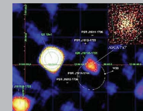
Cosmic Accelerators from keV to TeV
