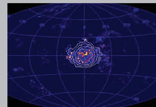
Evidence of Matter and Antimatter from the Galaxy Centre
