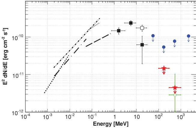
Figure 3. Spectrum of PSR B1509–58 from soft X-rays to \gamma -rays. 2\sigma upper limits derived with gtlike from LAT observations are represented by red stars. The green diamond represents the integrated flux derived from the light curves and estimates of the effective area and exposure in the 300 MeV–1 GeV energy range, as described in Section 4.1.2. The filled squares are the COMPTEL flux points derived from the excess counts in the 0.15–0.65 phase range, while the open square represents the 10–30 MeV flux in the 0.15–0.65 phase interval above the spatially determined background. The blue circles are the 2\sigma upper limits for the total fluxes obtained by EGRET. The different lines represent the best spectral fit measured by ASCA (short-dashed line, 0.7–10 keV), Ginga (dot-long-dashed line, 2–60 keV), CGRO-OSSE (long-dashed line, 50–750 keV), WELCOME (dotted line, 94–240 keV), and RXTE (dot-short-dashed line, 2–250 keV); see Kuiper et al. (1999) and references therein.
