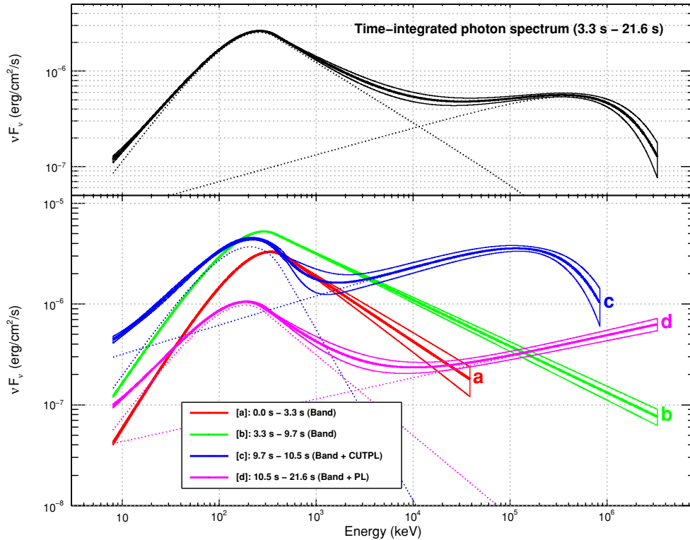
Figure 5. Top: the best-fit (Band+CUTPL) model for the time-integrated data plotted as a \nu F_\nu spectrum. The two components are plotted separately as the dashed lines, and the sum is plotted as the heavy line. The \pm 1\sigma error contours derived from the errors on the fit parameters are also shown. Bottom: the \nu F_\nu model spectra (and \pm 1\sigma error contours) plotted for each of the time bins considered in the time-resolved spectroscopy.
