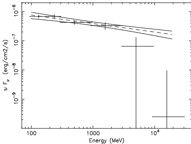
Figure 3. \nu F_\nu spectrum of the data points from the LAT-only unbinned likelihood analysis of GRB 090926A between T_0 + 3.3 s and T_0 + 21.6 s. Black dashed and solid lines show the best-fit power-law model and \pm 1\sigma error contours, derived from the covariance matrix of the fit.
