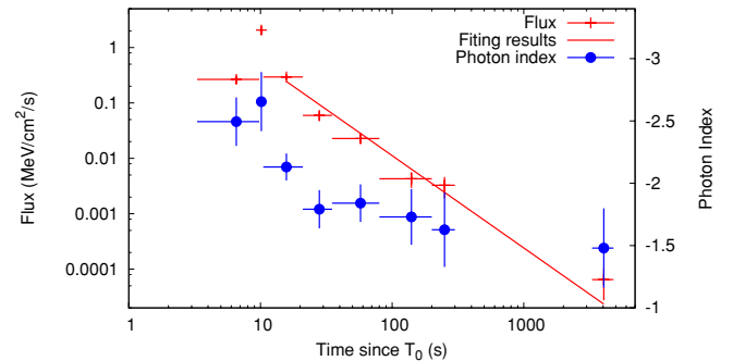
Figure 6. Time variation of the LAT flux (red cross) and photon index (blue filled circle) for the extended emission of GRB 090926A. After the end of the prompt emission at T_0 + 21.6 \text{ s} , the flux decays following a power law with index -1.69 \pm 0.03 (red solid line).
