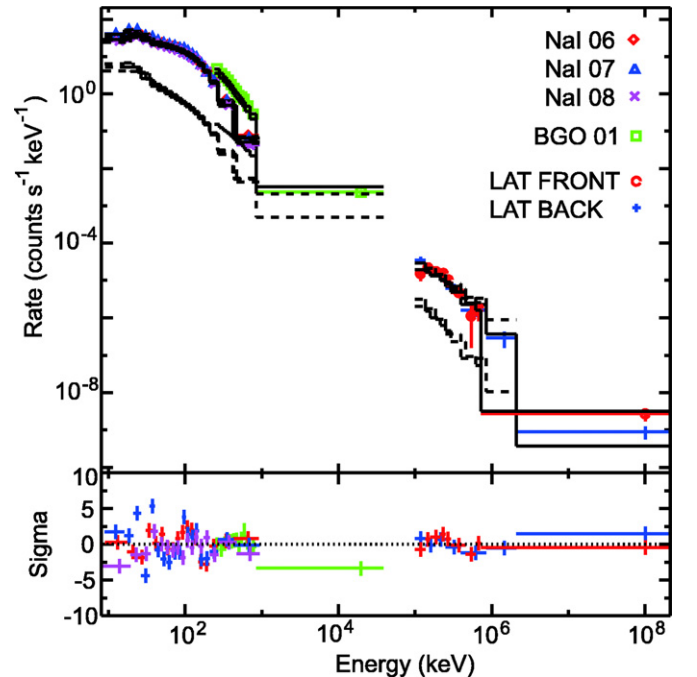
Figure 4. Joint spectral fitting of GBM and LAT data between T_0 + 3.3 s and T_0 + 21.6 s. The top panel shows the count spectra and best-fit (Band+CUTPL) model (histograms). The lower panel shows the residual of the spectral fitting.
