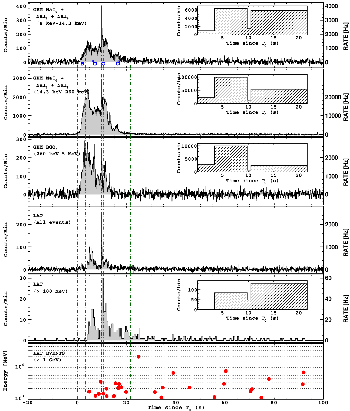
Figure 1. GBM and LAT light curves for the gamma-ray emission of GRB 090926A. The data from the GBM NaI detectors were divided into soft (8–14.3 keV) and hard (14.3–260 keV) bands to reveal similarities between the light curve at the lowest energies and that of the LAT data. The fourth panel shows all LAT events that pass the on-board GAMMA filter (Atwood et al. 2009). The first four light curves are background subtracted and are shown for 0.1 s time bins. The fifth and sixth panels show LAT data “transient” class events for energies >100 MeV and >1 GeV, respectively, both using 0.5 s time bins. The vertical lines indicate the boundaries of the intervals used for the time-resolved spectral analysis, T_0 + (0, 3.3, 9.8, 10.5, 21.6) s. The insets show the counts for each data set, binned using these intervals, to illustrate the numbers of counts considered in each spectral fit.
