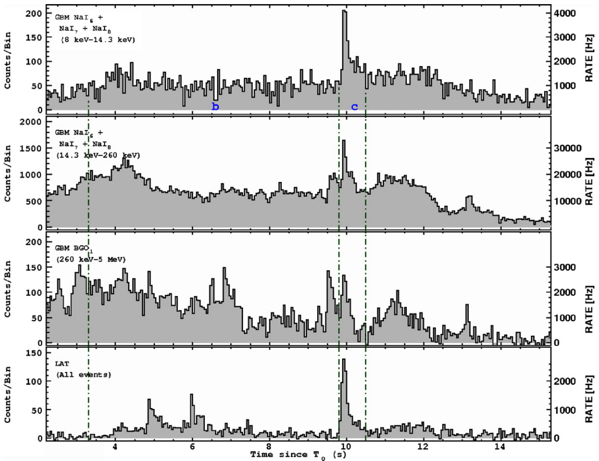
Figure 2. GBM and LAT light curves for the gamma-ray emission of GRB 090926A with 0.05 s time binning for the core of the prompt phase. The vertical dashed lines at T_0 + 9.8 s and T_0 + 10.5 s define interval c used in the spectral analysis, see Section 4.1.
