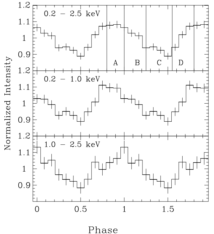
FIG. 1.—EPIC PN light curve of 1E 1207–5209 for three different energy ranges. The vertical lines in the top panel indicate the intervals used for the phase-resolved spectroscopy.
