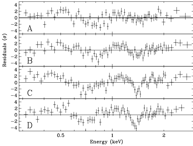
FIG. 3.—Phase-resolved spectroscopy. The four panels show the residuals of blackbody fits with N_{\text{H}} fixed at 3 \times 10^{20} \text{ cm}^{-2} for the phase intervals labeled on Fig. 1.
