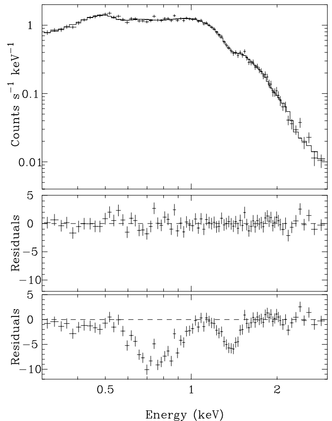
FIG. 2.—Fit of the PN data with a blackbody plus power law and two Gaussian lines. In the upper panel the data are compared with the model folded through the instrumental response. The middle panel shows the residuals in units of sigma. The lowest panel shows the residuals obtained by removing the lines from the model.
